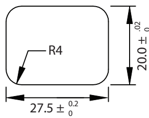
PANEL CUTOUT
