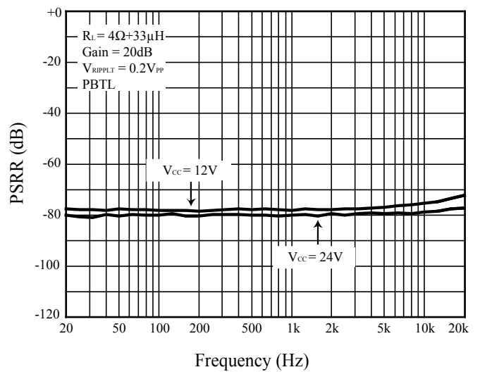
Figure 18 PSRR
