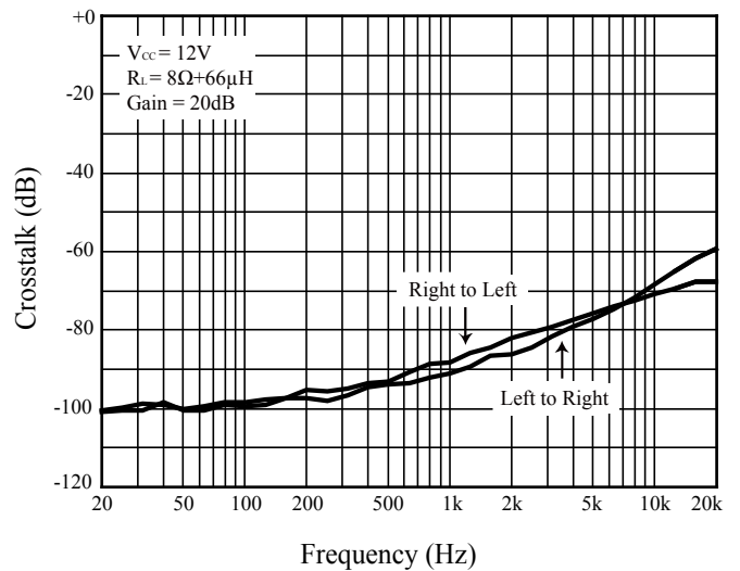
Figure 20 Crosstalk
