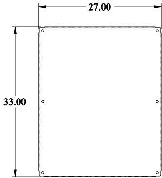
INNER PANEL
