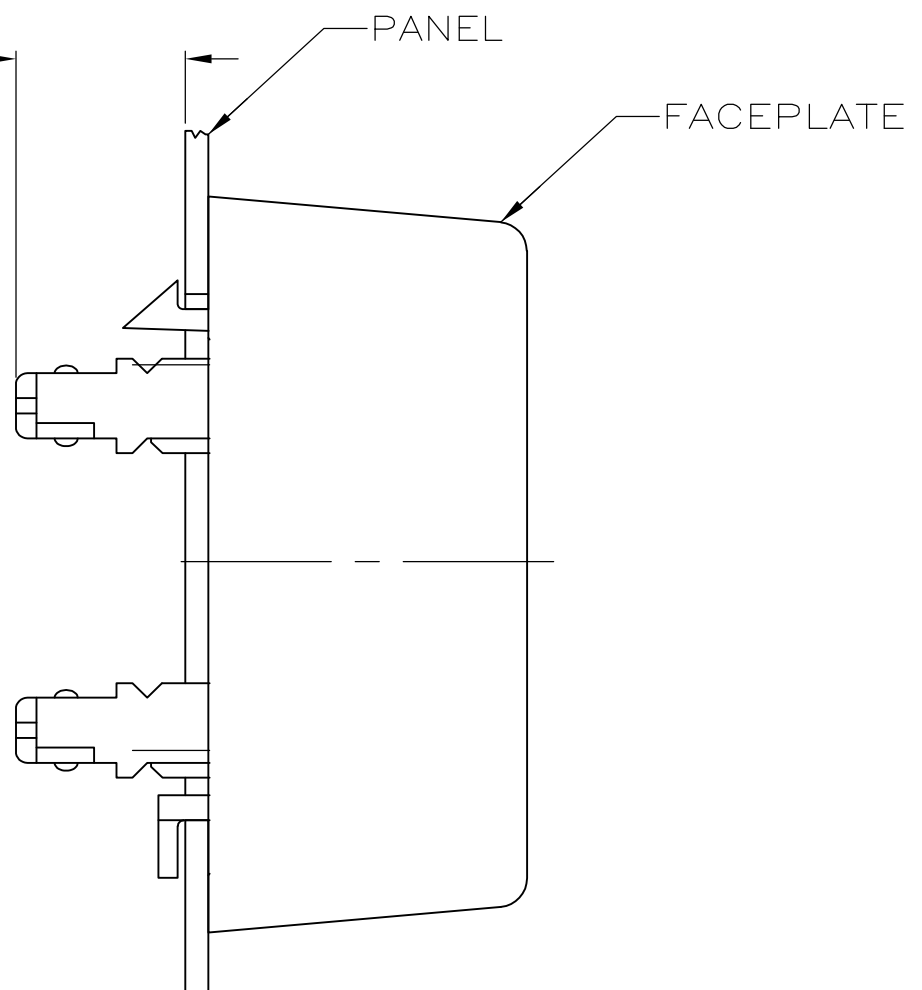
SUGGESTED MOUNTING
