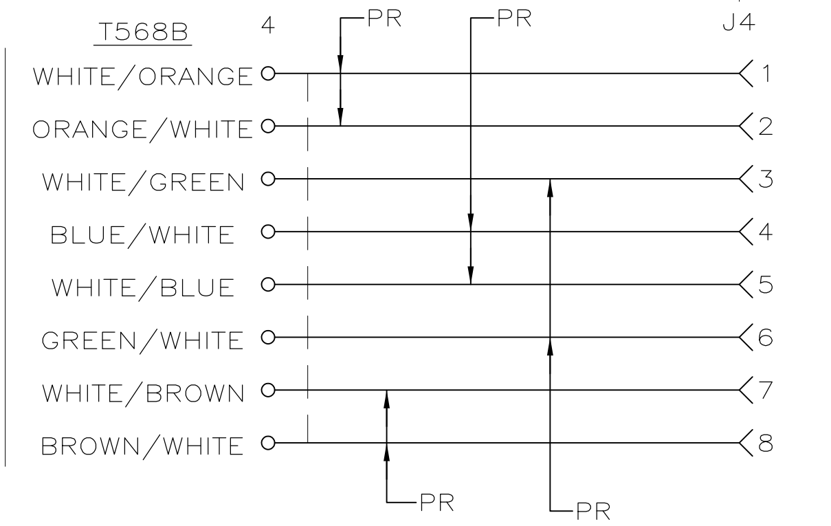
ELECTRICAL SCHEMATIC FOR T568A OR T568B WIRING PATTERN
