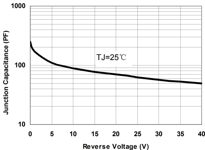
Fig.1-Typical Junction Capacitance
