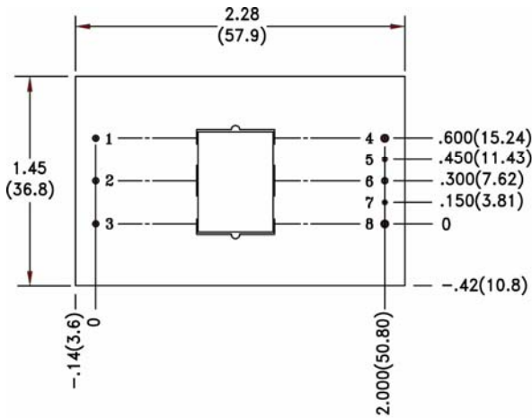
PIN VIEW
