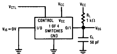
FIGURE 5. t_{PZL} , t_{PLZ} Propagation Delay Time Control to Signal Output
