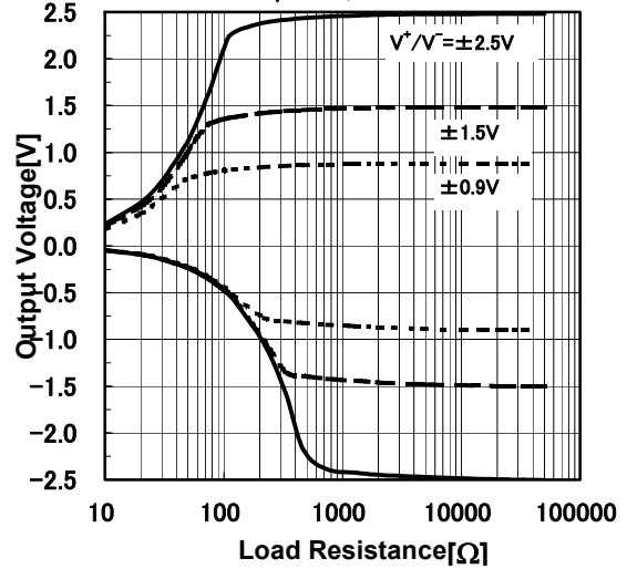
Output Voltage vs. Load Resistance ( V^+/V^- )
