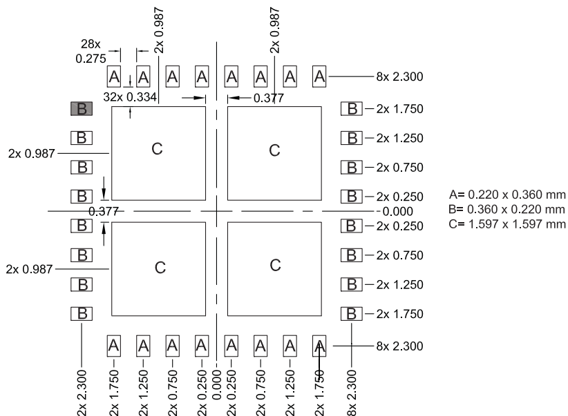
Figure 2. Stencil Recommendation
