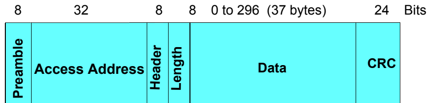
Figure 4. Packet structure
