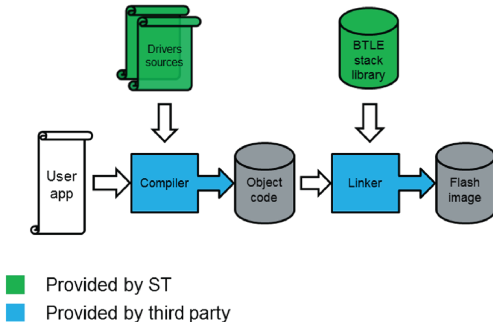
Figure 9. BLE stack reference application
