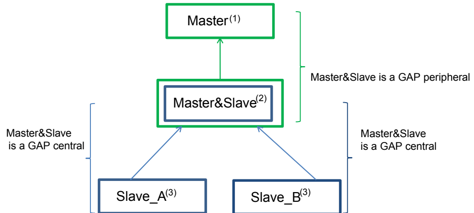
Figure 11. BLE simultaneous master and slave scenario
