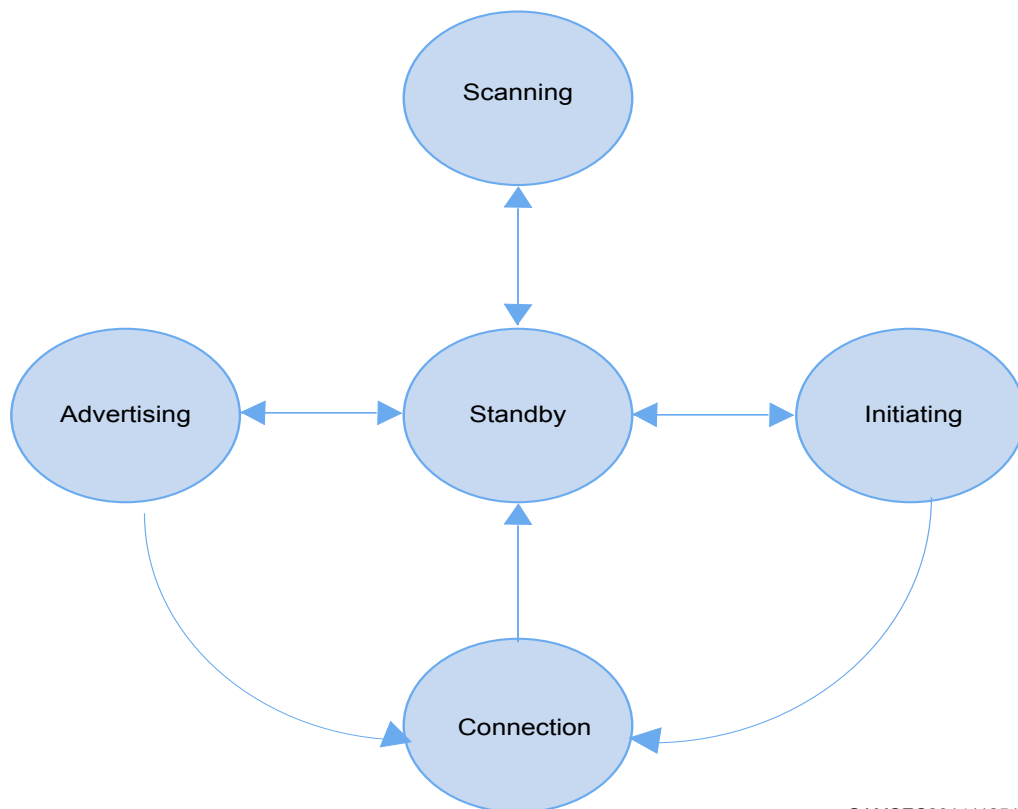
Figure 3. Link Layer state machine
