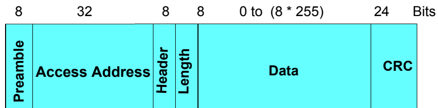
Figure 5. Packet structure with LE data packet length extension feature
