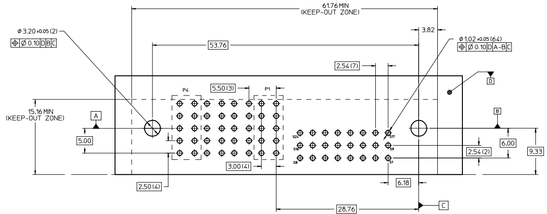
RECOMMENDED PC BOARD LAYOUT & KEEP-OUT ZONE
