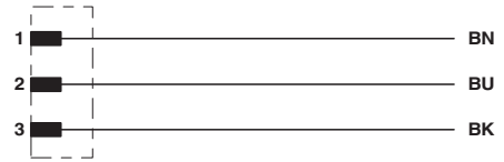
Contact assignment of the DEUTSCH DT04-3P
