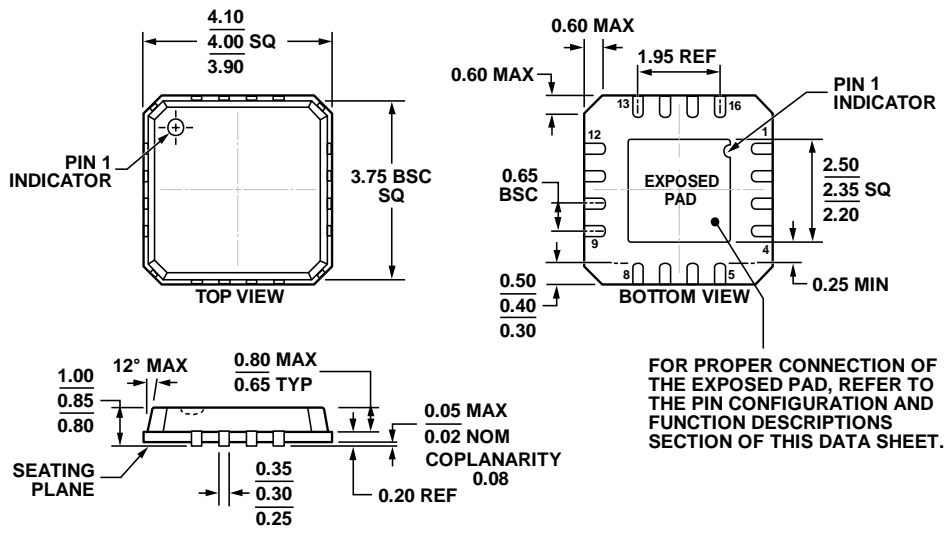
Figure 40. 16-Lead Lead Frame Chip Scale Package [LFCSP_VQ] 4 mm × 4 mm Body, Very Thin Quad (CP-16-10) Dimensions shown in millimeters
