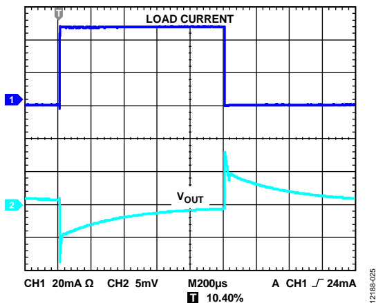
Figure 29. Load Transient Response, C_{IN} = C_{OUT} = 1\text{ }\mu\text{F} , I_{LOAD} = 1\text{ mA to }50\text{ mA} , 200\text{ ns Rise Time} , CH1 = \text{Load Current} , CH2 = V_{OUT}
