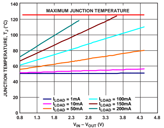
Figure 54. 100 mm 2 of PCB Copper, LFCSP, T A = 50°C
