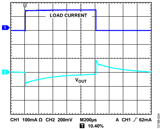
Figure 28. Load Transient Response, C_{IN} = C_{OUT} = 1\text{ }\mu\text{F} , I_{LOAD} = 1\text{ mA to }150\text{ mA} , 200\text{ ns Rise Time} , CH1 = \text{Load Current} , CH2 = V_{OUT}
