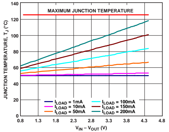
Figure 53. 500 mm 2 of PCB Copper, LFCSP, T A = 50°C
