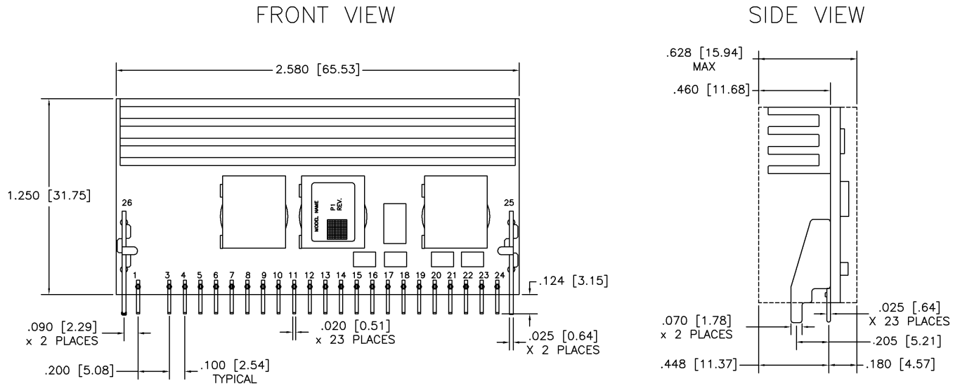
Figure 11. Mechanical Drawing
