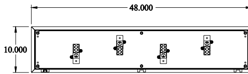
FRONT VIEW - COVER REMOVED
