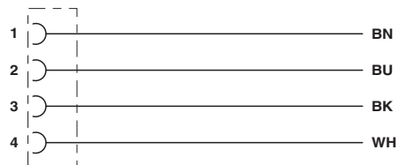
Contact assignment of the DEUTSCH DT06-4S
