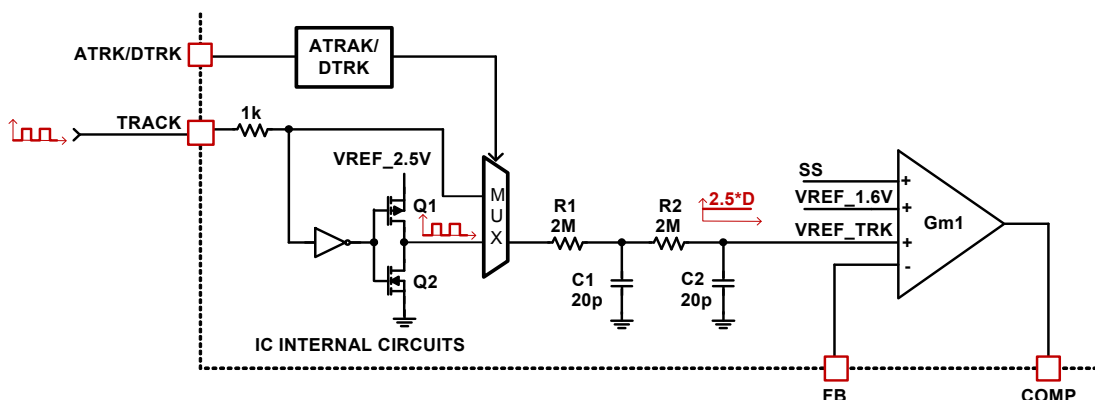
FIGURE 51. TRACK FUNCTION BLOCK DIAGRAM
