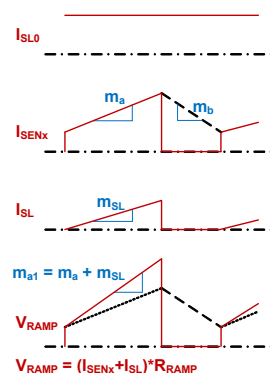
FIGURE 61. SLOPE COMPENSATION BLOCK DIAGRAM
