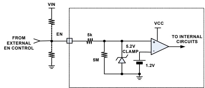
FIGURE 59. ENABLE BLOCK
