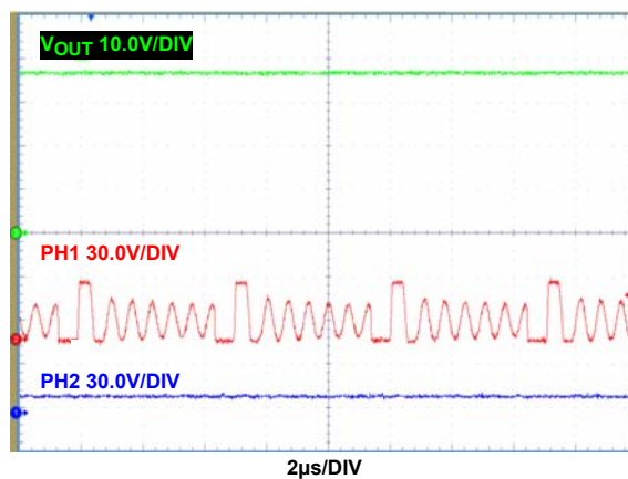
FIGURE 20. DE+PH_DROP MODE ( DE/PHDRP = FLOAT ), PH1 DIODE EMULATION WITH PH2 DROPPED, I_{OUT} = 29mA
