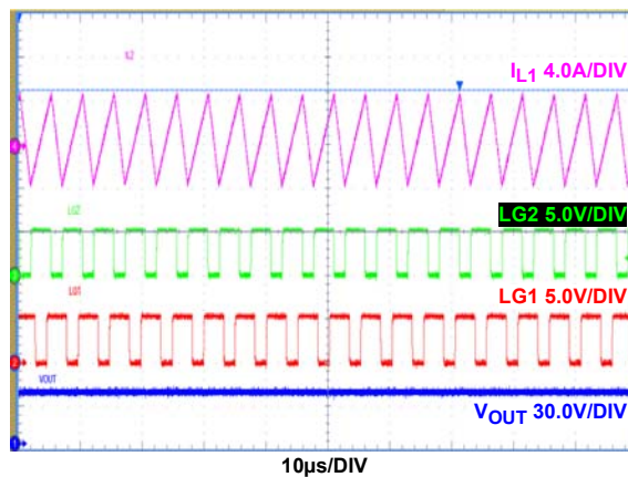
FIGURE 16. CCM MODE (DE/PHDRP = GND), PHASE 1 INDUCTOR RIPPLE CURRENT, I_{OUT} = 0A
