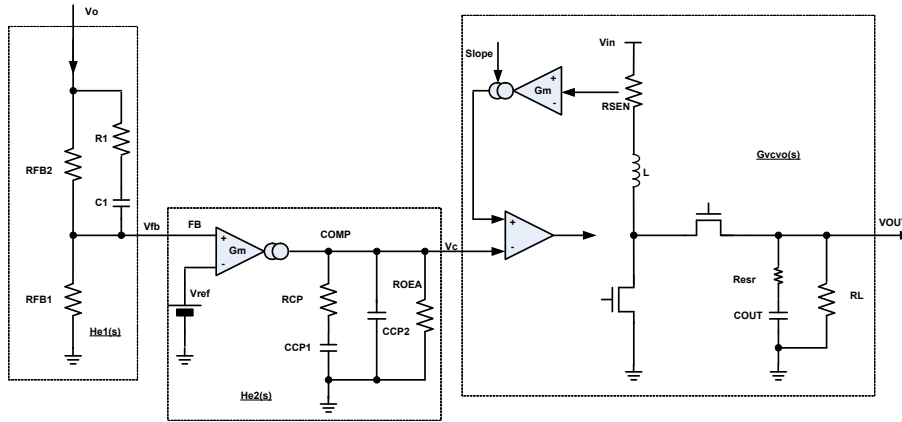
FIGURE 64. CONCEPTUAL BLOCK DIAGRAM OF PEAK CURRENT MODE CONTROLLED BOOST REGULATOR
