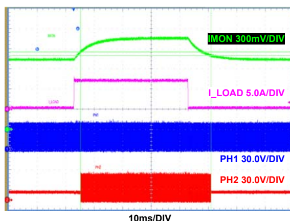
FIGURE 22. DE+PHDRP MODE ( DE/PHDRP = FLOAT ), PH2 ADDED AND DROPPED, UNDER TRANSIENT STEP LOAD OF 1A TO 8A
