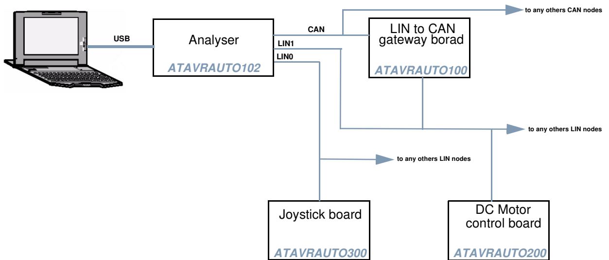
Figure 1-1. Evaluation kit
