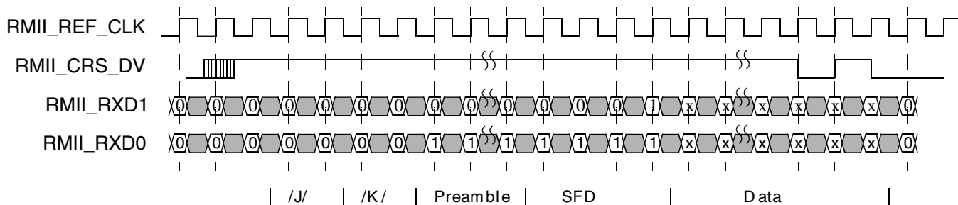
Figure 46-69. RMII receive operation
