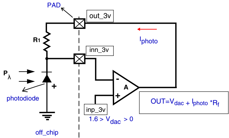
Figure 38-6. Reverse-Biased Application Diagram
