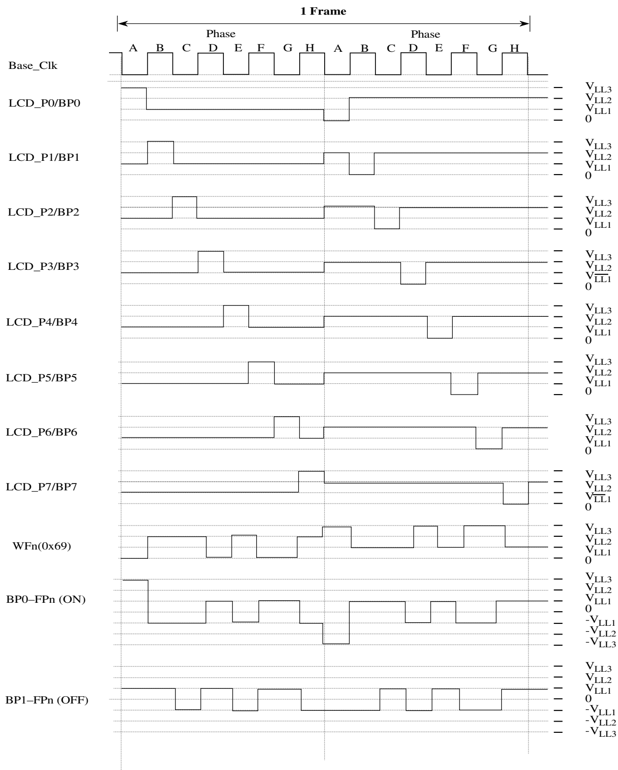
Figure 57-31. 1/8 Duty and 1/3 bias (low-power waveform)
