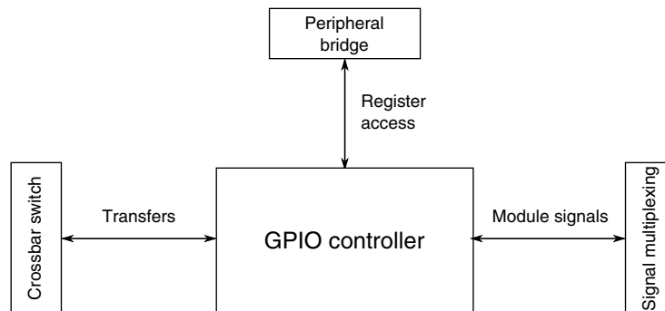
Figure 3-66. GPIO configuration
