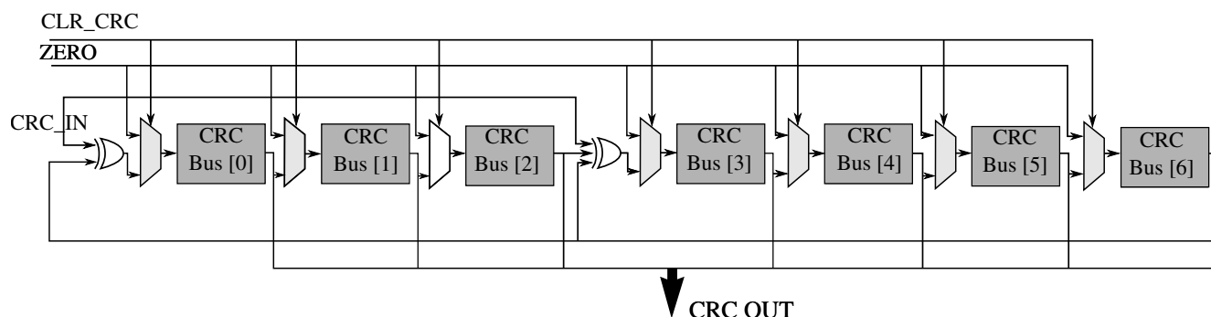
Figure 53-34. Command CRC Shift Register
