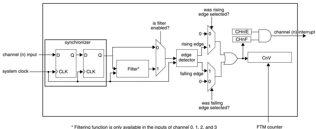
Figure 41-175. Input Capture Mode
