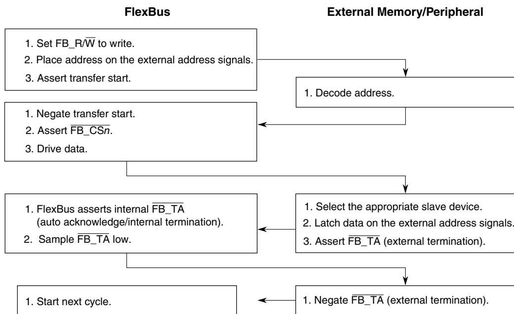
Figure 29-28. Write-Cycle Flowchart
