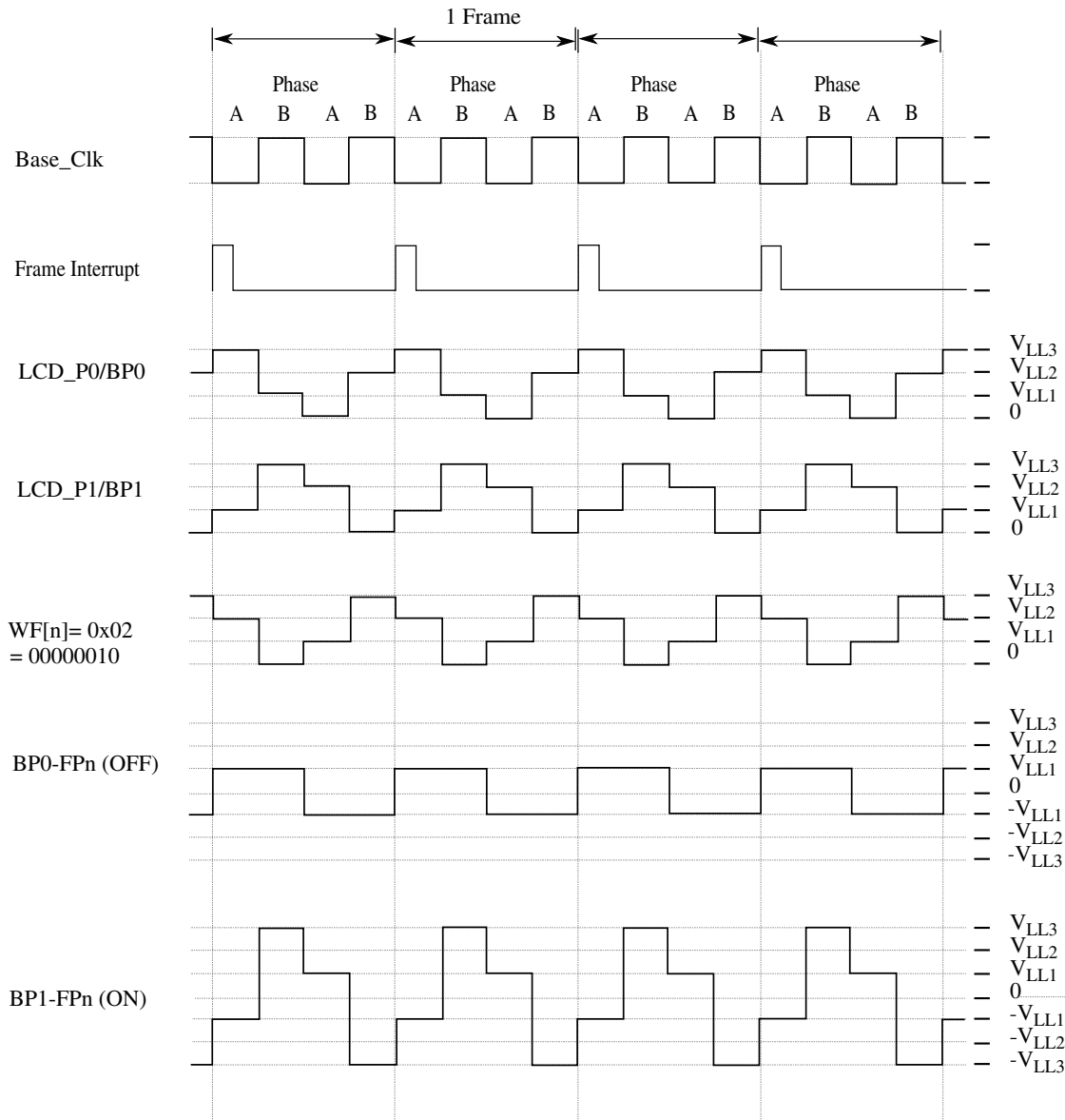
Figure 57-29. 1/2 Duty and 1/3 bias (low-power waveform)
