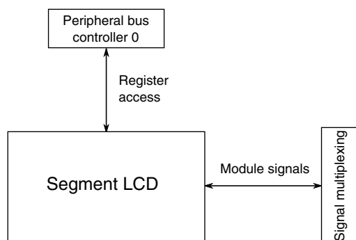
Figure 3-68. SLCD configuration
