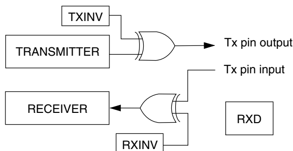
Figure 52-241. Single-wire operation (C1[LOOPS] = 1, C1[RSRC] = 1)
