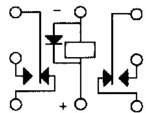
TERMINAL VIEW
