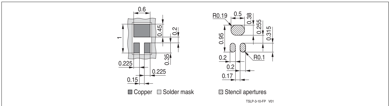
Figure 9-2 Package Footprint
