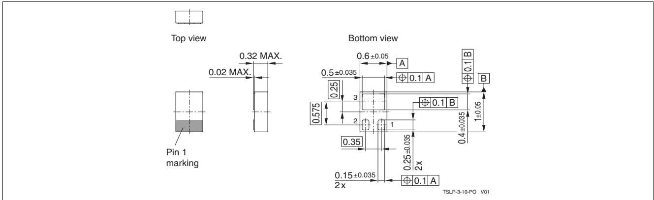
Figure 9-1 Package Outline
