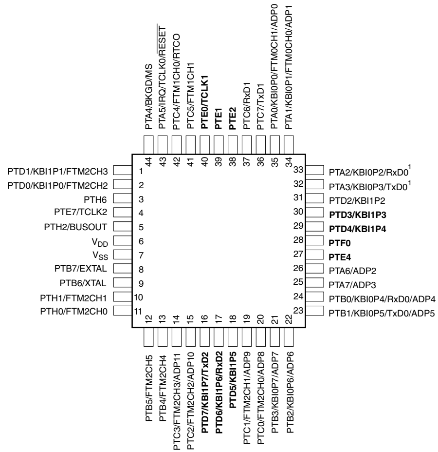
Figure 14. MC9S08PL60 44-pin LQFP package
