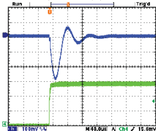
Step Load Transient Response (Vin=12V, Vout=1.8V, Cload=12x10µF X5R 0805 ceramic, total 120µF, Iout=0A to 1.5A) Top trace=Vout, Bottom trace=Iout
