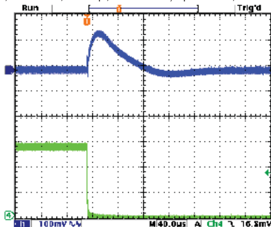
Step Load Transient Response (Vin=12V, Vout=3.3V, Load=10x10µF 5R 0805 ceramic, plus 1x470µF, 7mΩ POSCAP, total 570µF, Iout=1.5A to 0A) Top trace=Vout, Bottom trace=Iout
