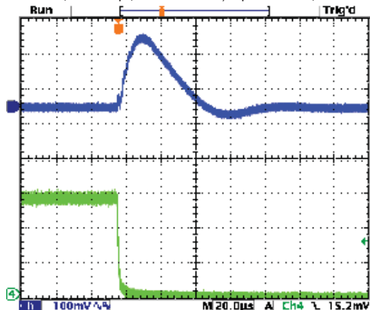
Step Load Transient Response (Vin=5.5V, Vout=3.3V, Load=10x10µF X5R 0805 ceramic, plus 1x470µF, 7mΩ POSCAP, total 570µF, Iout=1.5A to 0A) Top trace=Vout, Bottom trace=Iout
