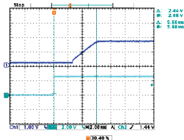
On/Off Enable Startup (Vin=12V, Vout=1.5V, Iout=1.5A, Clod=0) Channel 2=Enable, Channel 1=Vout
