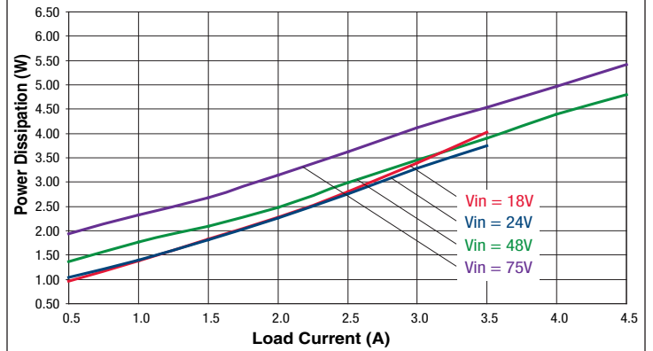
Power Dissipation vs. Load Current @ 25°C
