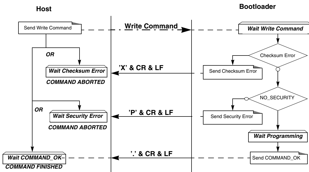
Figure 24-13. Write/Program Flow
