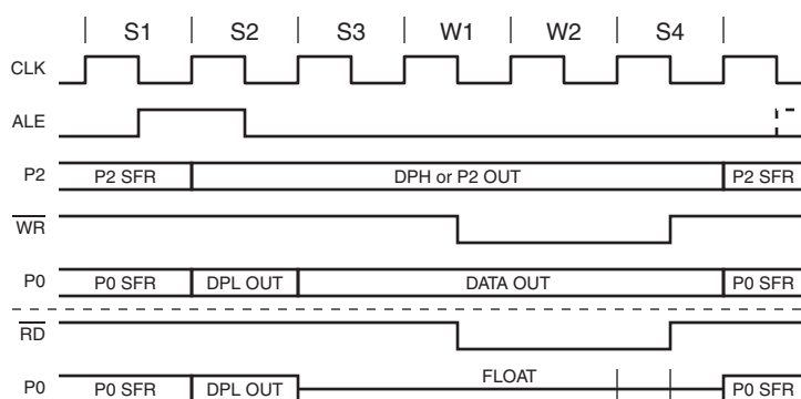
Figure 3-14. MOVX with Two Wait States (WS = 10B)
