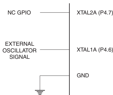
Figure 6-4. External Clock A Drive Configuration
