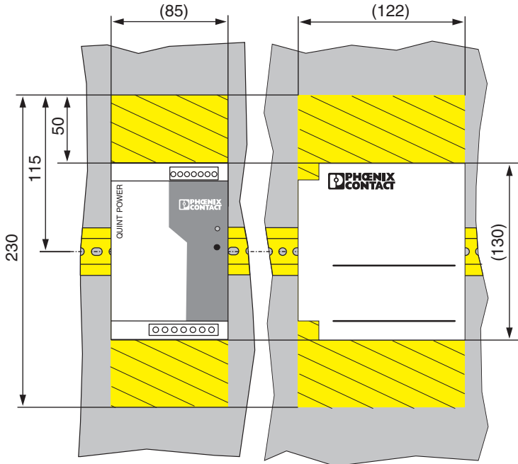
Figure 4 Mounting position (dimensions in mm)
