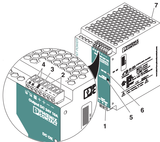
Figure 1 Operating elements
