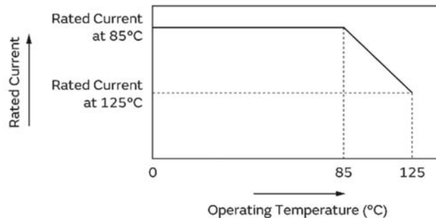
Derating of Rated Current
