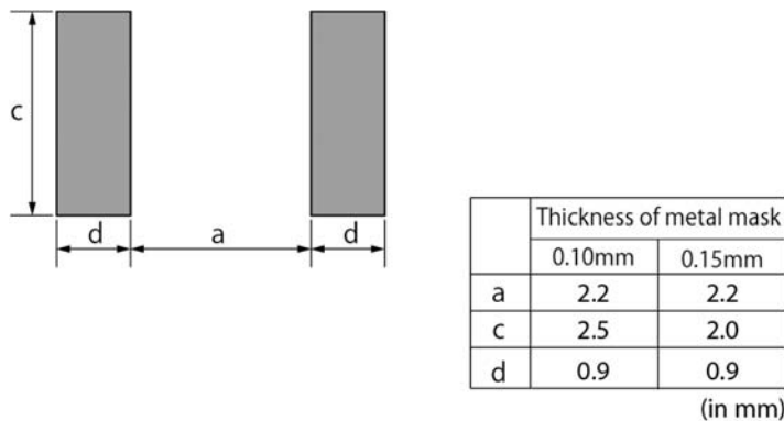
Metal mask aperture pattern
